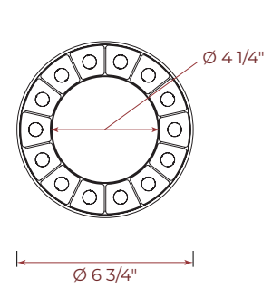
TLMW - Trimless millwork
