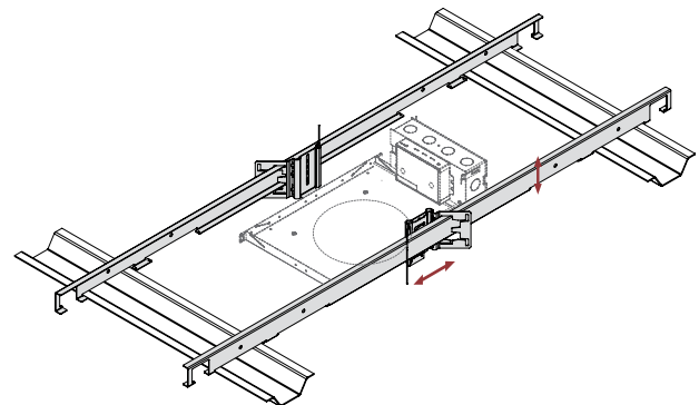
AHC - Adjustable Hat Channel Bars
