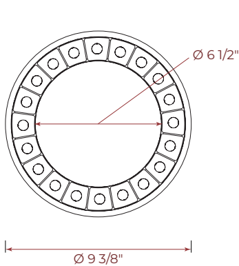
TRM - Flanged trim
