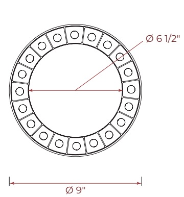
TLMW - Trimless millwork
