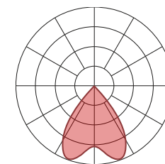
Precision Specular Optic
