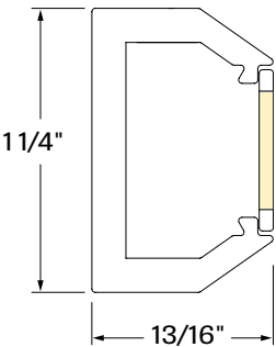
SECTION VIEW
