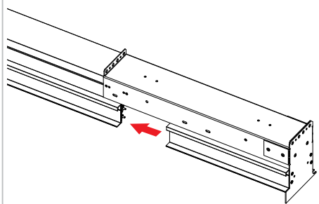
STEP 6 - RECONNECT SLEEVE BASE TO FIXTURE
