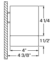
1.5" Drop Lens 1
